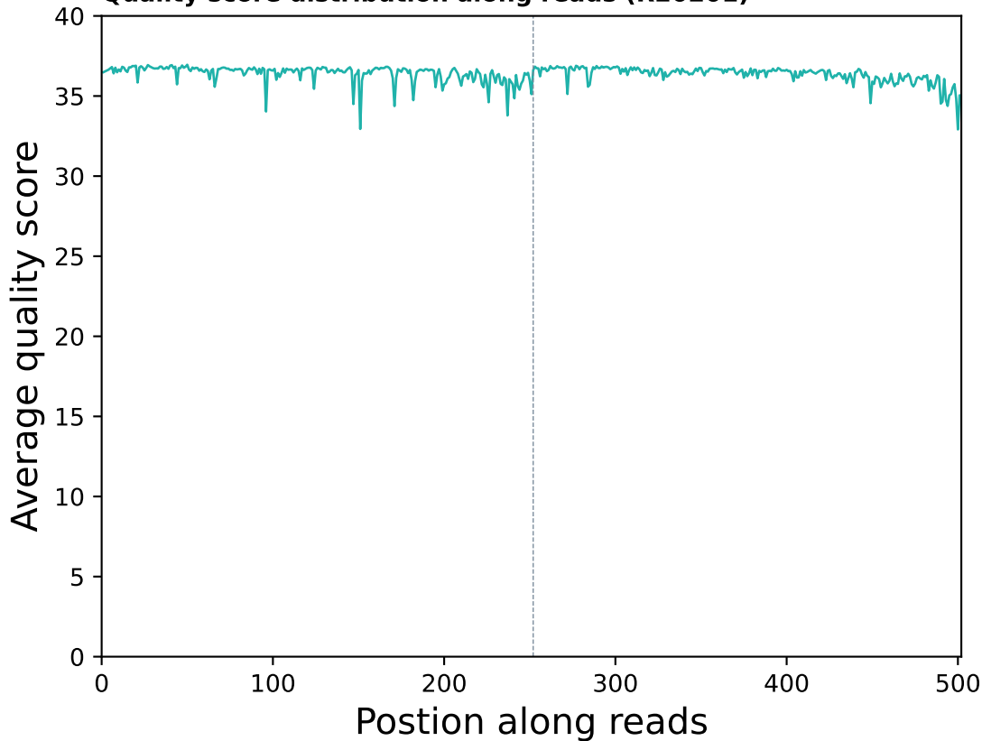
Quality score distribution along reads (R20201)
